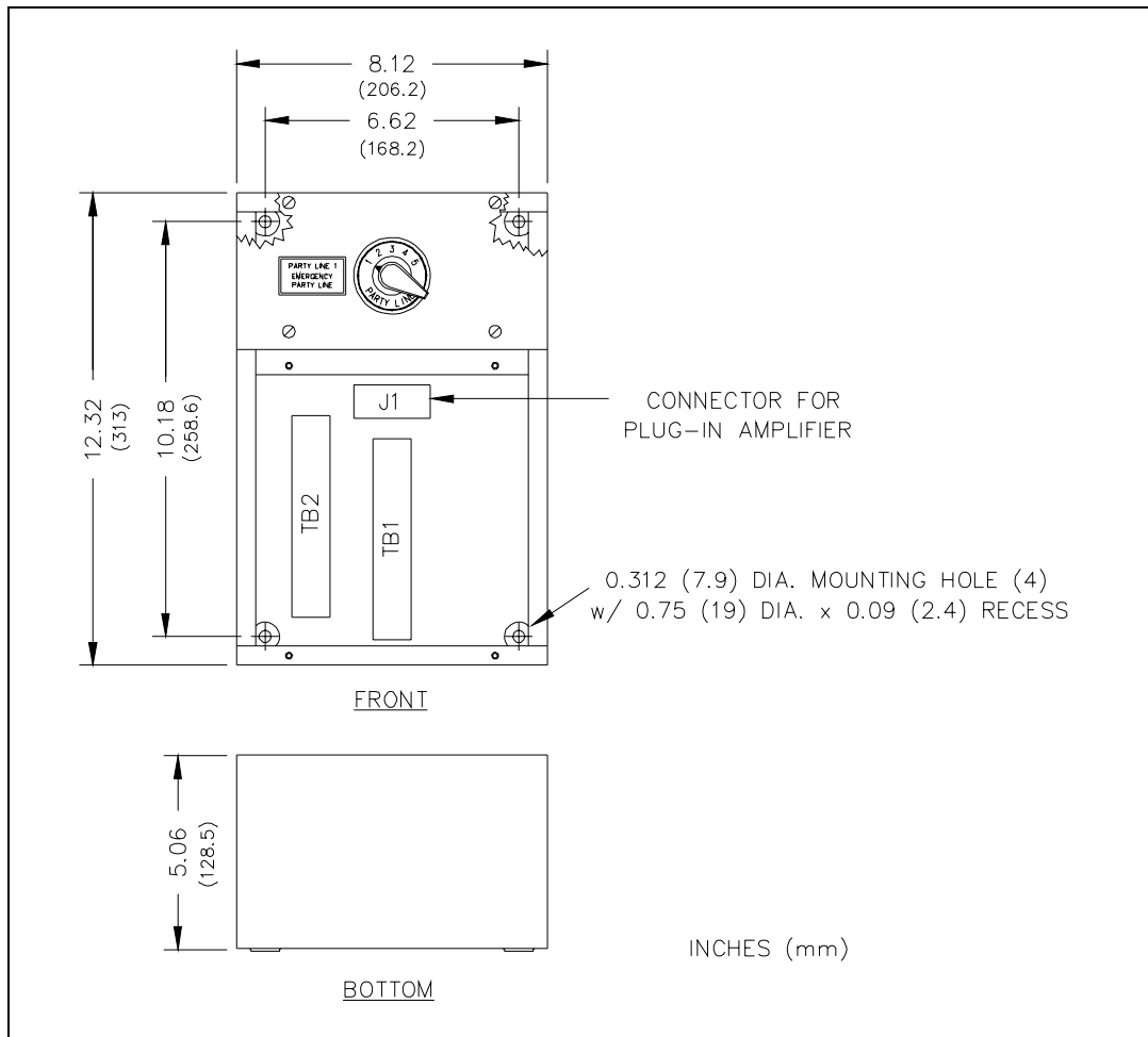
Figure 1. Indoor Enclosure Mounting
