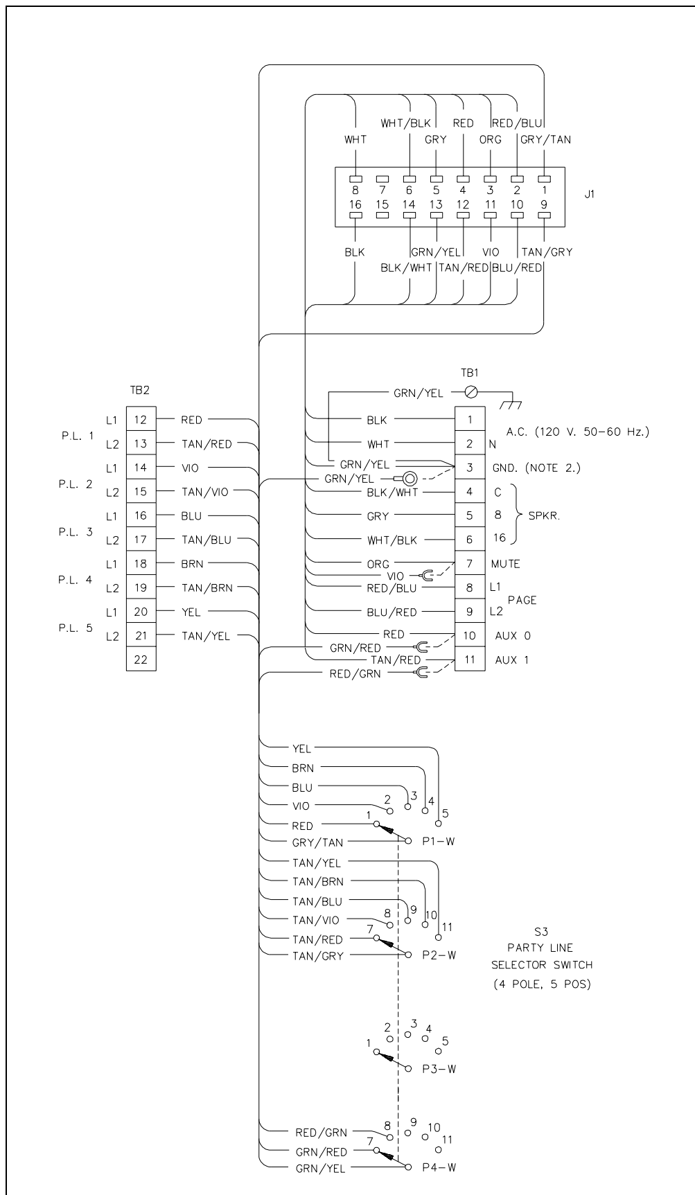
Figure 2. Wiring Diagram
